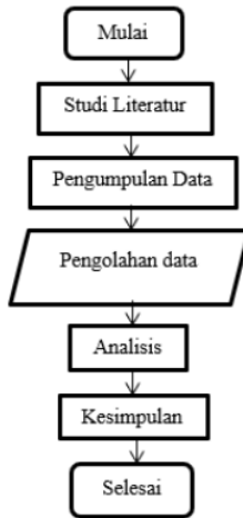
Gambar 2. FlowChart Penelitian
