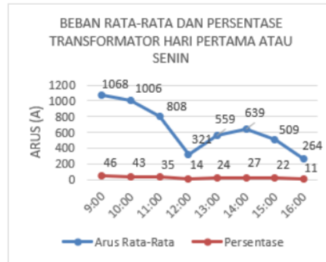
Gambar 3. Grafik Beban Rata-Rata & Presentase Hari Senin
