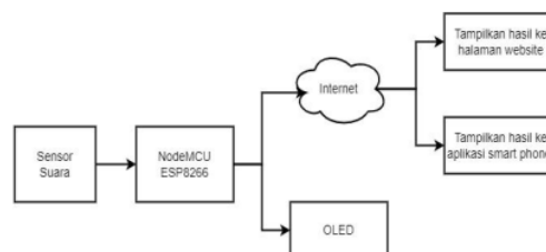
Gambar 3. 1 Diagram Blok Alat
