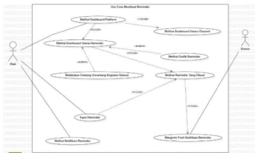
22 Gambar 2. Diagram Use Case Reminder Kegiatan
