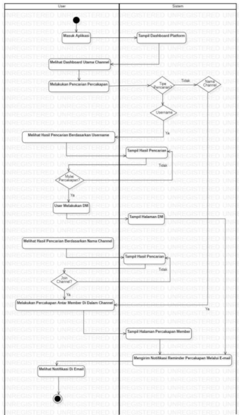
Gambar 6. Diagram Activity Pencarian Channel
