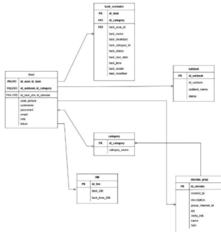
Gambar 10. Entity Relationship Diagram
