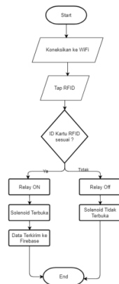
Gambar 3 Flowchart
