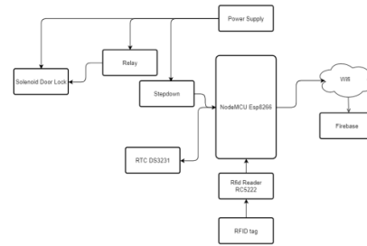
Gambar 4 Blok Diagram
