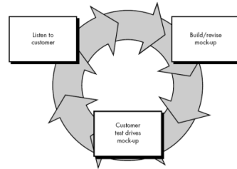
Gambar 1 Alur Penelitian
