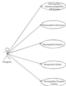
11 Gambar 1 Usecase Diagram
