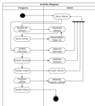
Gambar 2 Activity Diagram
