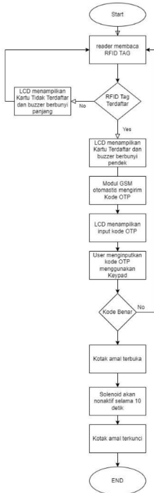
Gambar 2. 3 Flowchart Sistem
