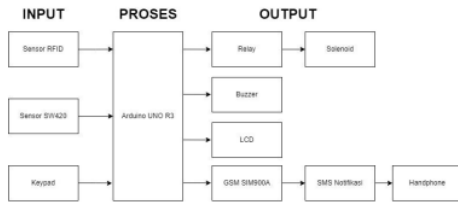
Gambar 2. 2 Blok Diagram
