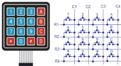
Gambar 1. 8 Keypad
