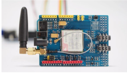
Gambar 1. 3 Modul GSM SIM900A
