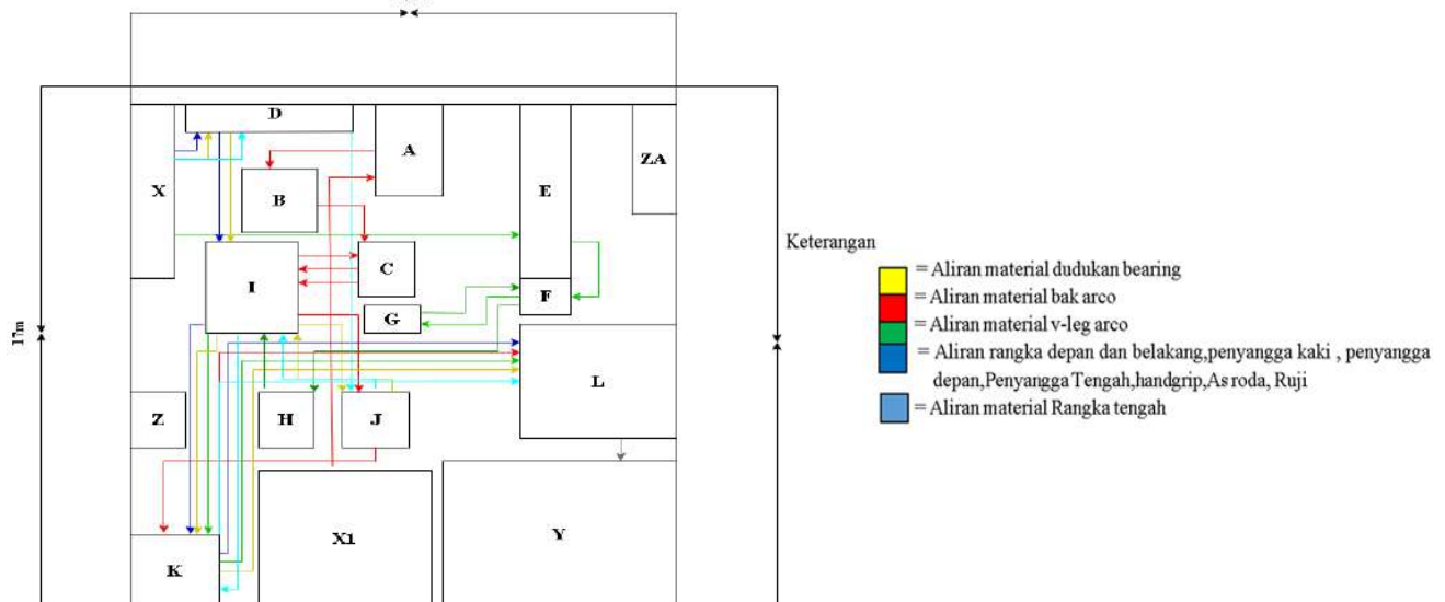
Gambar 1 Layout awal
