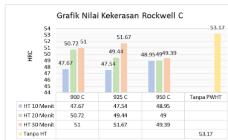
Gambar 15. Nilai Kekerasan Rockwell C
