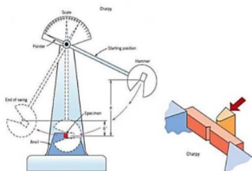
Gambar 3. Sketsa Uji Impact Charpy
