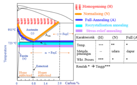
Gambar 2. Diagram Temperatur Normalizing
