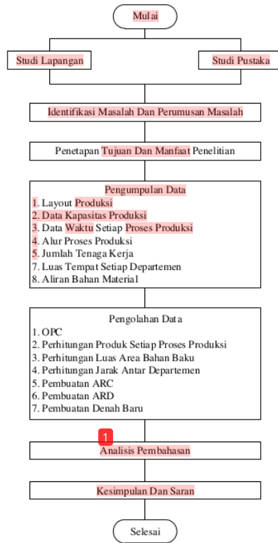
Gambar 3. Flowchart Penelitian
