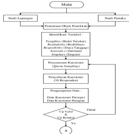
Gambar 2. Flowchart Penelitian
