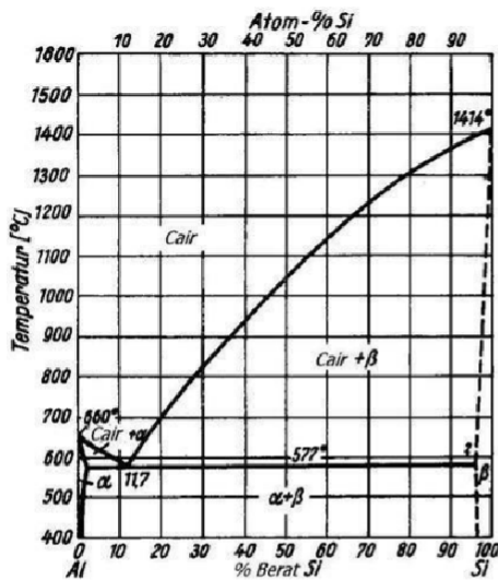
Gambar 1. Diagram Fasa
