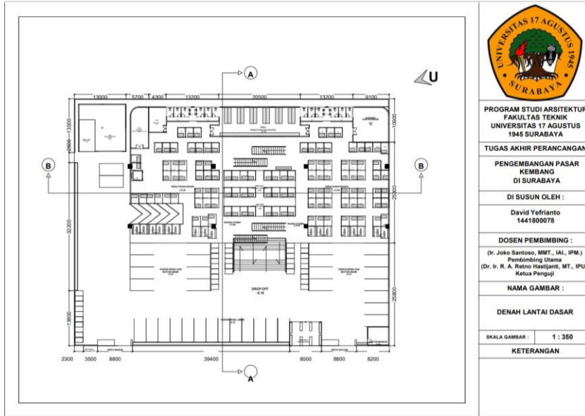
Gambar 70 Denah lantai 1
