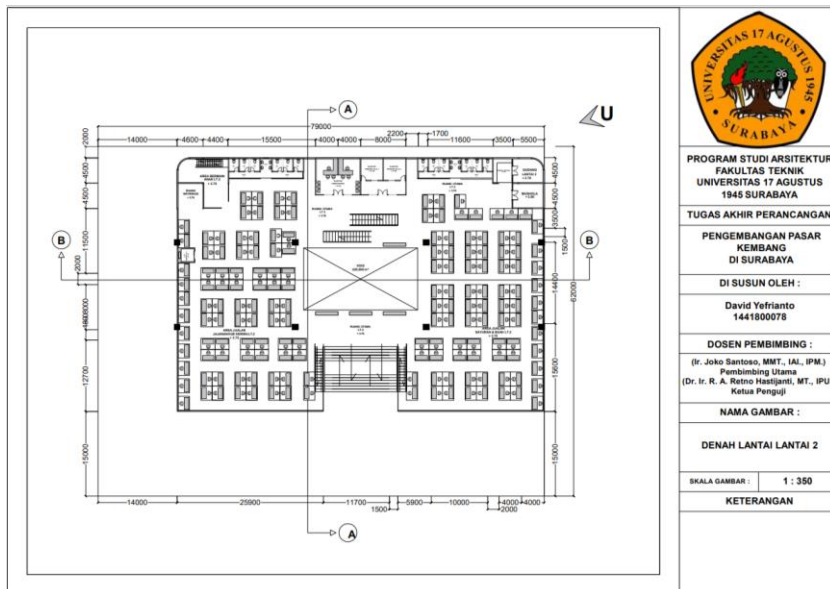
Gambar 71 Denah Lantai 2
