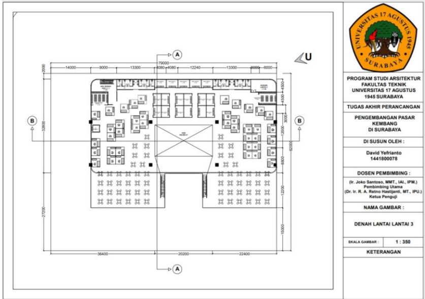
Gambar 72 Denah Lantai 3
