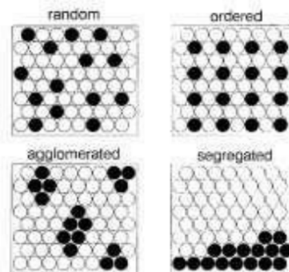
Gambar 1. Difersi Campuran Bubuk Al-Cu
