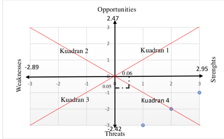
Gambar 4.8 Diagram IFAS-EFAS
