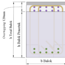
Gambar 5. Penampang Balok Half Precast
