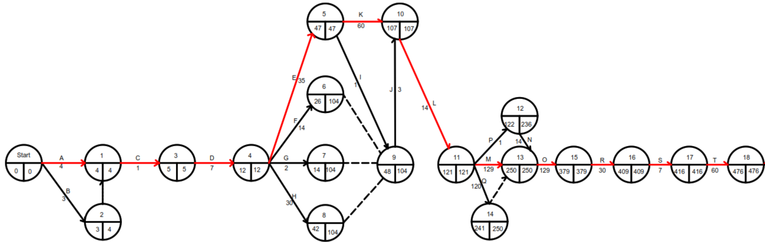
Lampiran 1 : Diagram Network Planning Durasi Normal (Manual)
