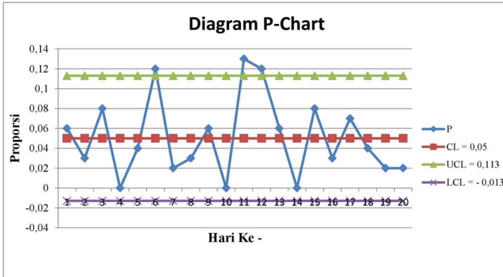
Gambar 1 : Diagram peta kendali (P-Chart)
