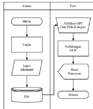
Gambar 2. Flowchart Diagram
