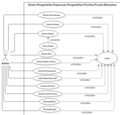
Gambar 3 Usecase Diagram
