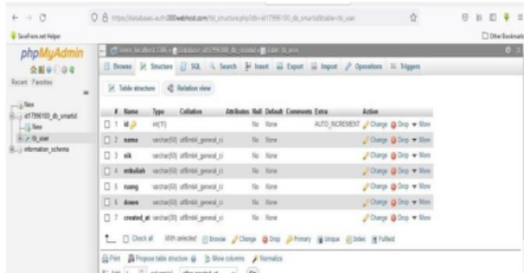
Gambar 3.4 Database
