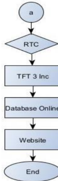
Gambar 2.5 Flowchart System
