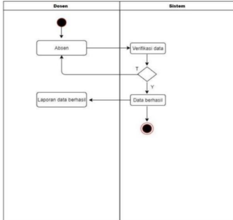
Gambar 2.8 Activity Diagram Dosen
