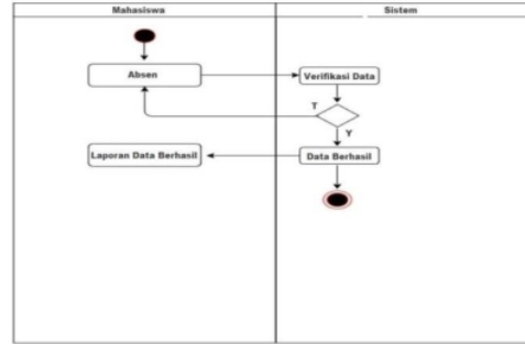
Gambar 2.9 Activity Diagram Mhs
