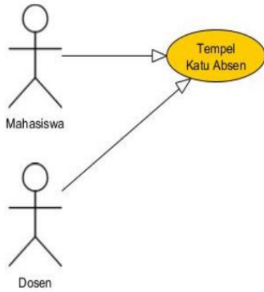
Gambar 2.7 Use Case
