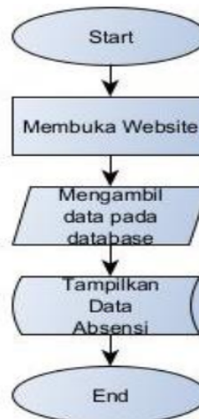
Gambar 2.6 Flowchart Website
