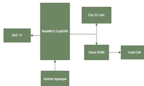
Gambar 3.1 Diagram Blok
