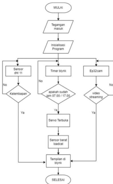
Gambar 3.2 Flowchart
