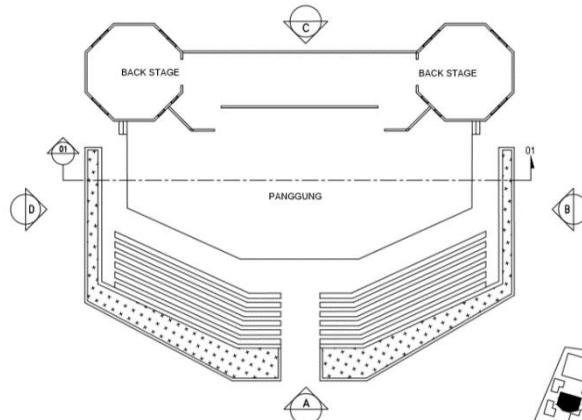
DENAH AMPITHEATER Skala 1:125
