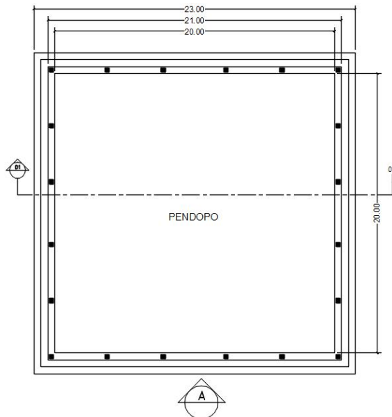
DENAH PENDOPO Skala 1:125
