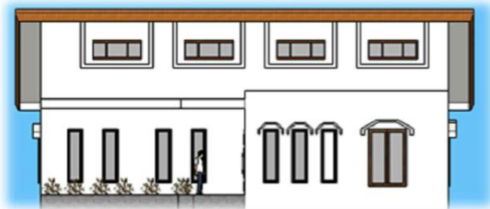
TAMPAK VIEW A Skala 1:125
