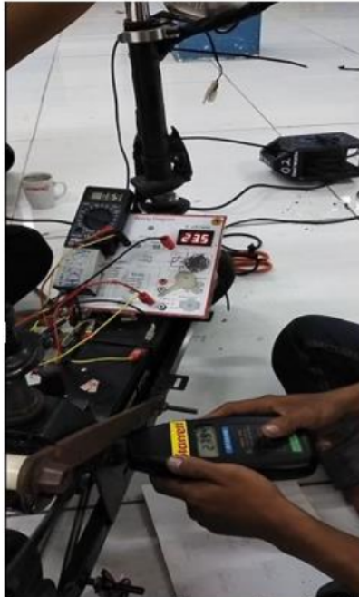
pengujian alternator diameter 65mm Rpm 2700
