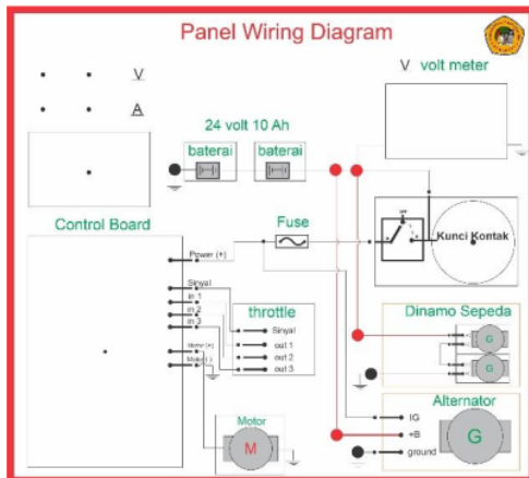
Panel wiring diagram kelistrikan
