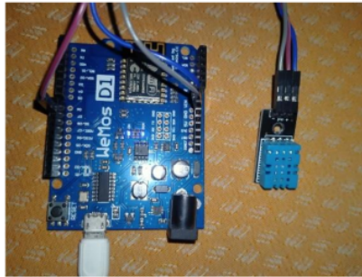
Gambar 7 DHT11
