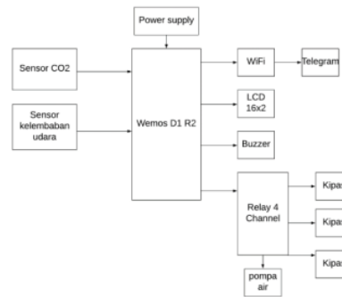
Gambar 1 Blok Diagram
