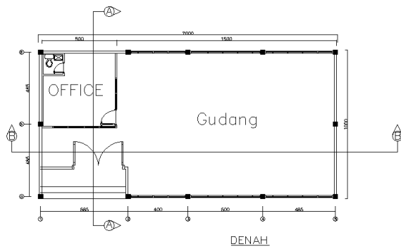
Denah Massa 7
