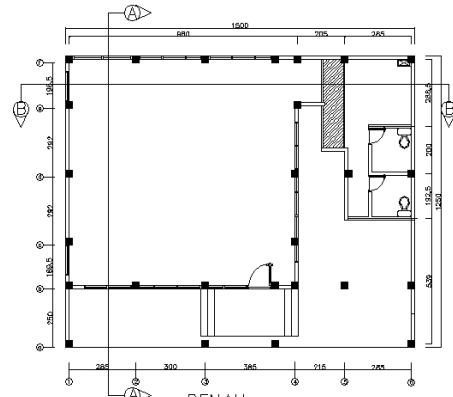
DENAH
