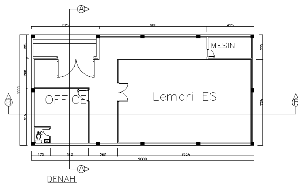
Denah Massa 6
