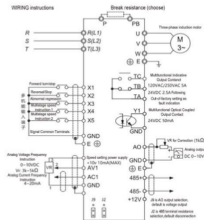
Gambar 3.3 Wiring diagram Inverter
