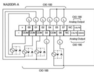
Gambar 3.7 Diagram Wiring Output PLC Omron CP1E NA20DR-A
