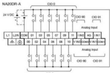
Gambar 3.6 Diagram Wiring Input PLC Omron CP1E NA20DR-A
