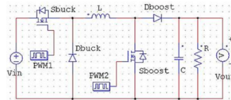
Gambar 2.1 Buck Boost Converter
