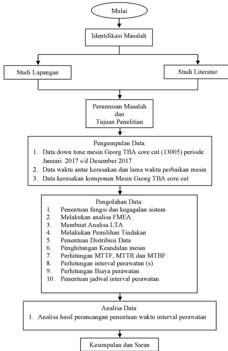
Gambar 1. Flowchart Penelitian
