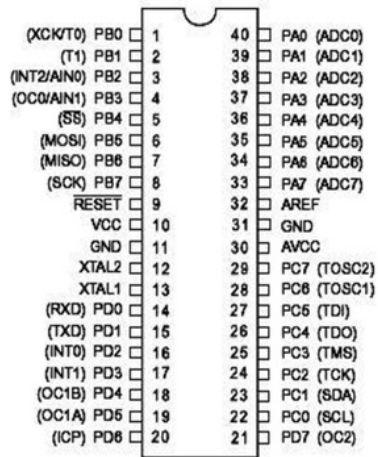
Gambar 4 Port-Port ATmega 16
