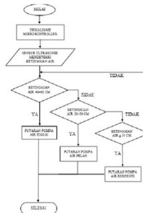
Gambar 13 Flowchart Program
