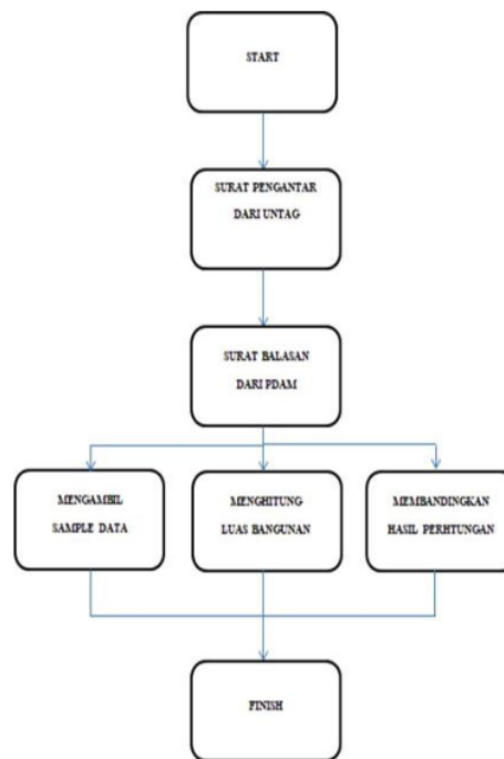
Gambar 3.1 Diagram Penelitian
