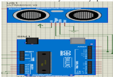
Gambar 3. 2 Rangkaian Sensor Ultrasonic HC-SR04
