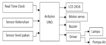
Gambar 3. 1 Diagram blok
