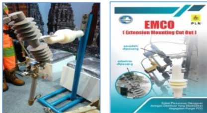
Gambar 3.4.1 Extension Mounting Cut Out (EMCO)
