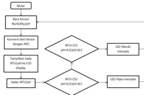
Gambar 3.2 Flowchart
