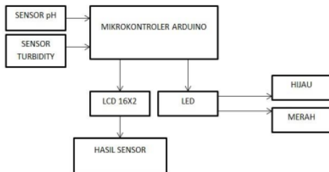
Gambar 3.1 Blok Diagram
