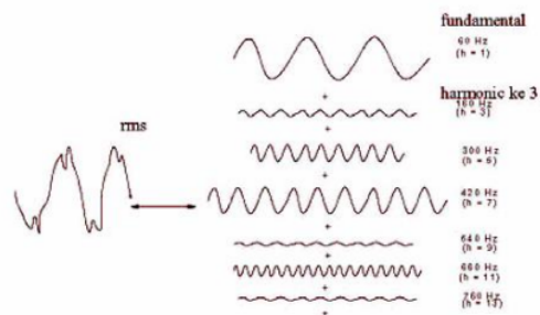
Gambar 1. Harmonisa
