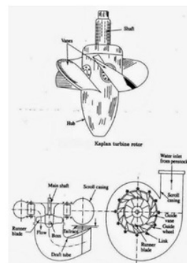
Gambar 1. Turbin Kaplan [6]
