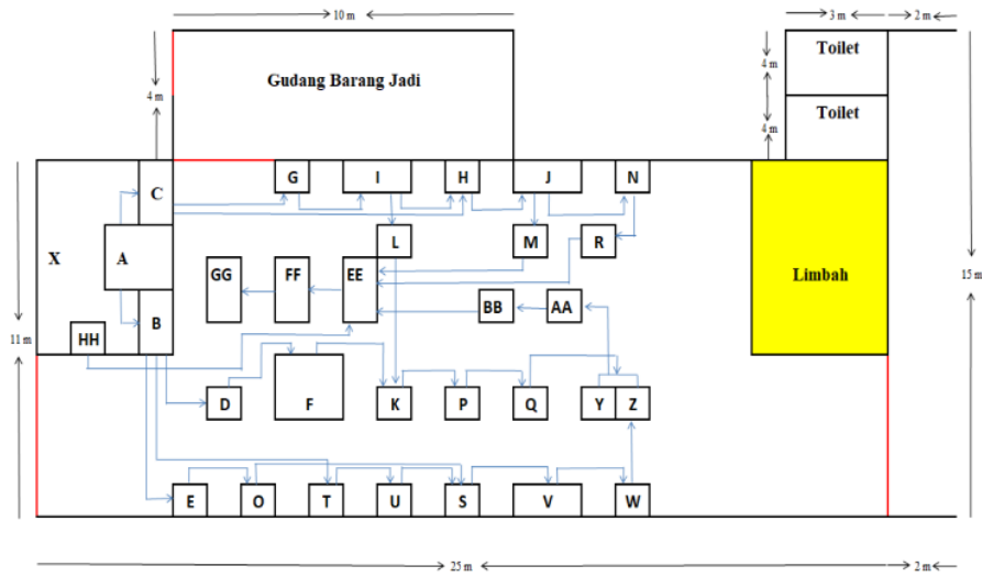
Gambar 4.6 Layout Usulan
