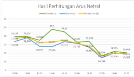
Gambar 10 Diagram Hasil Perhitungan Arus Netral
