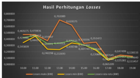
Gambar 11 Diagram Besar Losses
