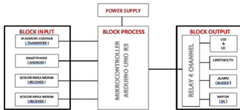
Gambar 3.1 Blok Diagram
