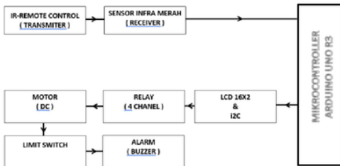
Gambar 3.2 SUB Blok Diagram IR Remote (Transmitter)
