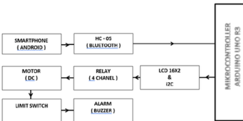
Gambar 3.3 SUB Blok Diagram Smartphone (Android)
