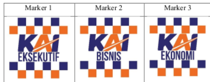
Gambar 4. Marker
