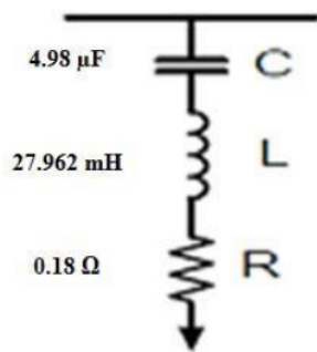
Gambar 7. Desain Filter Single Tuned SDP 2 Fasa R
