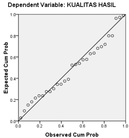
Normal P-P Plot of Regression Standardized Residuals
