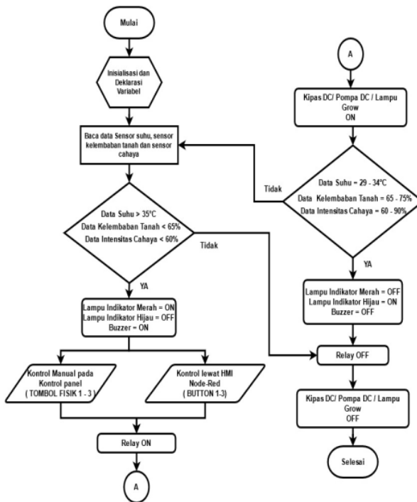
Gambar 3.3 Flowchart Sistem Kontrol Indoor Garden System
