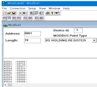
Gambar 4.4 Data Modbus
