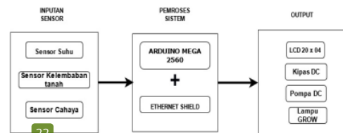
Gambar 3.1 Blok Diagram Hardware
