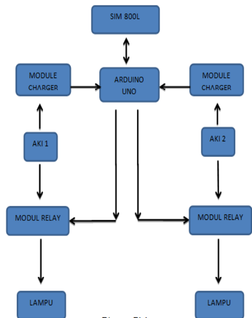
Diagram Blok
