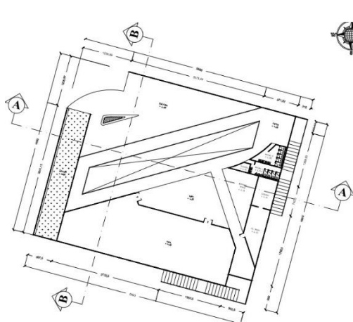
Denah Massa Galeri Lt. 2
