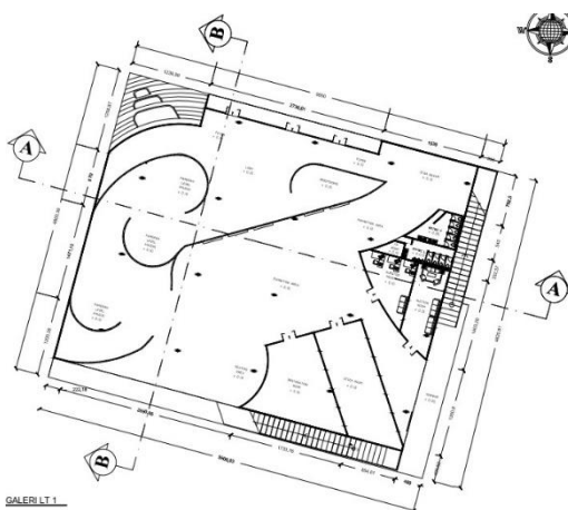
Denah Massa Galeri Lt. 1
