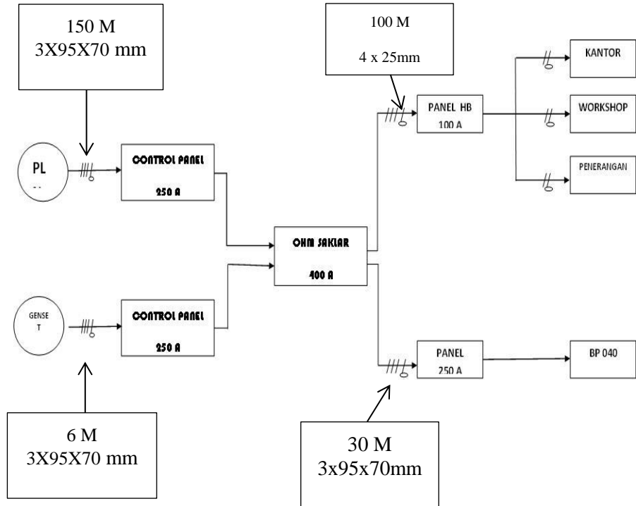
Diagram line listrik BSP Sidoarjo
