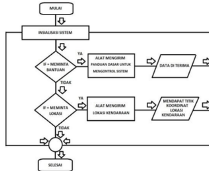
3.2.1 Gambar Flowchart system software
