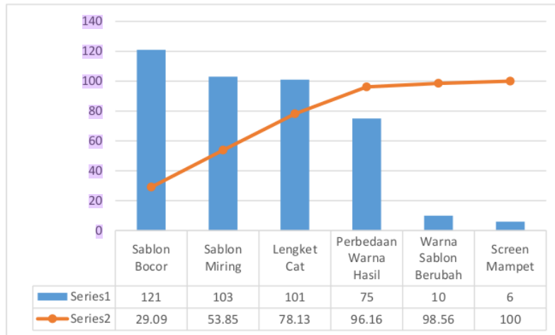
Gambar 8. Diagram Pareto
